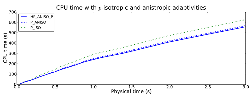
Figure 19: Cumulative CPU times as a function of physical time for multi-mesh configurations with P_ISO, P_ANISO, and HP_ANISO_P adaptivity modes.
