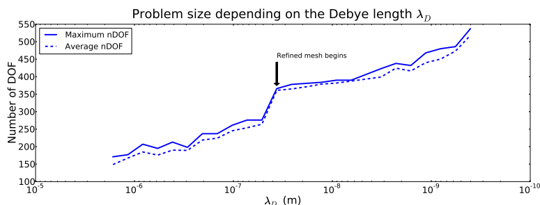
Figure 24: Problem size depending on the Debye length. Initially the coarse mesh (shown in Fig. 6(a)) was used. It was necessary to use the fine mesh (see Fig. 6(c)) for smaller \lambda_D values.
