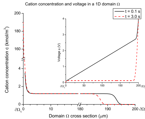
Figure 2: Sample concentration C and voltage \phi in a 1D domain \Omega \subset \mathbb{R} . Dirichlet boundary conditions ( V_{\partial\Omega_1} = 0V and V_{\partial\Omega_2} = 4V ) were applied to the Poisson equation (1.2) and Neumann conditions to the Nernst-Planck equation (1.1).
