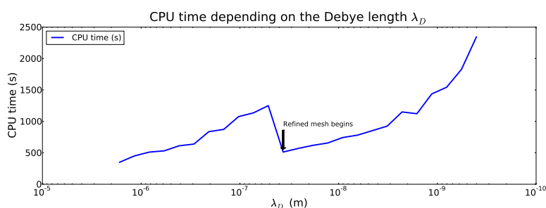
Figure 25: CPU time depending on the Debye length. Initially the coarse mesh (shown in Fig. 6(a)) was used. It was necessary to use the fine mesh (see Fig. 6(c)) for smaller \lambda_D values.
