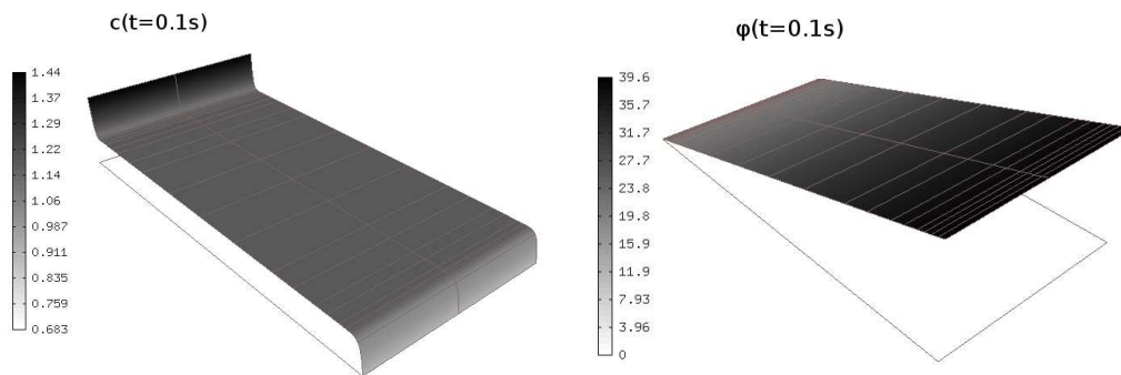
Figure 7: Scaled concentration c and voltage \varphi at t=0.1s .
