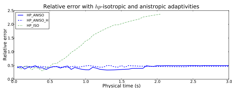
Figure 17: Relative solution error as a function of physical time for multi-mesh configurations with HP_ANISO, HP_ANISO_H, and HP_ISO adaptivity modes.
