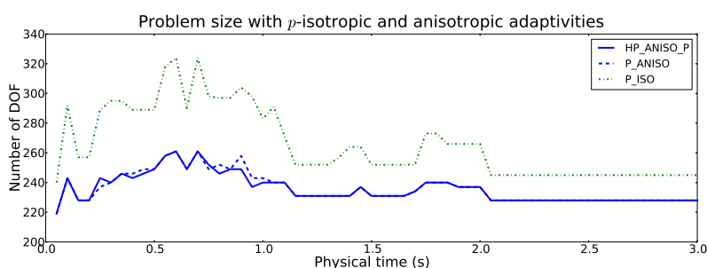
Figure 18: Number of DOF as a function of physical time for multi-mesh configurations with P_ISO, P_ANISO, and HP_ANISO_P adaptivity modes.
