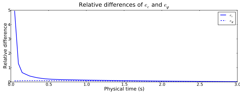
Figure 20: Relative difference e_c^n and e_\varphi^n .
